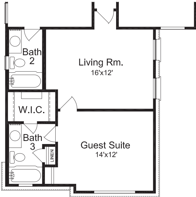
Guest Suite/ Bath 3 Option
