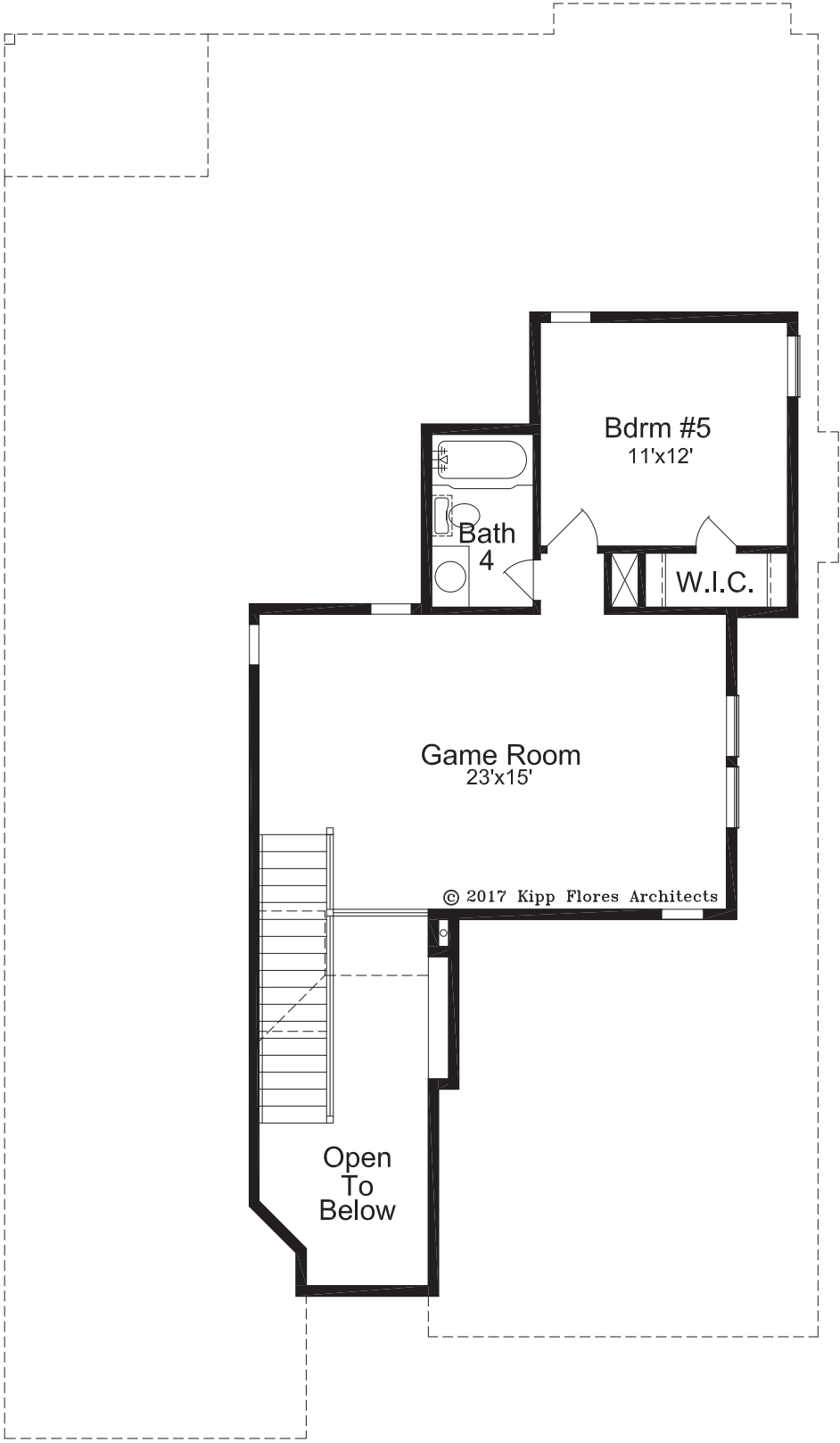
Optional Second Floor Plan
